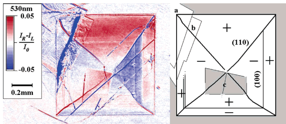
Figure 6. CD micrograph at 530 nm of a thin (<50 nm) DHA crystal showing clearly the (110) and (100) twin planes between enantiomorphous domains. Regions a and b are thin, overlaid crystallites. Region c shows an intergrown crystal with a superposition of enantiomorphous domains ((001) twinning) that may reveal a nascent pinwheel of the kind observed in thicker samples (Figure 4e and f). The streaks are due to scratches and needles of a metastable polymorph.
